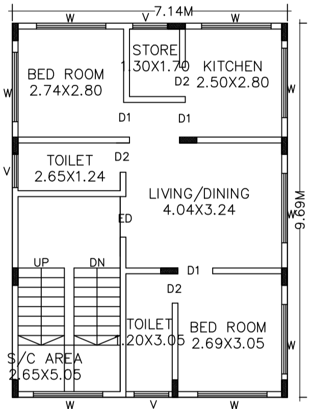
TYPICAL FIRST & SECOND FLOOR PLAN
