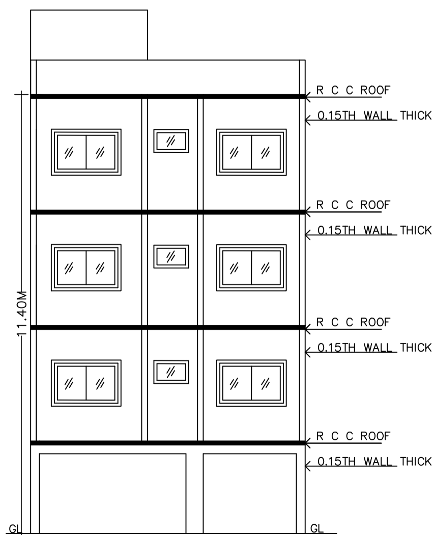
SECTION X-X
